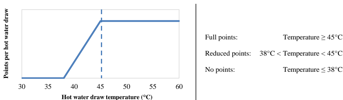
Figure 9 Scoring function for the Hot Water Subcontest
