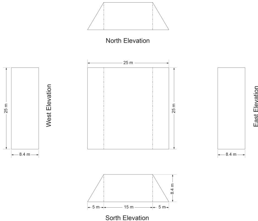
Figure 13 Solar envelope dimensions (meter)
